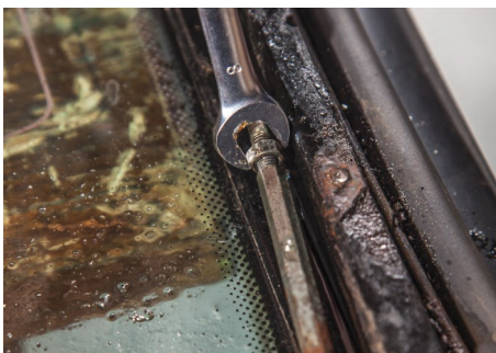
9. Unscrew the rod locknut, and unscrew the catch adjuster. The catches may need prising off the tailgate as you expose more threads, so strip easily when corroded.
